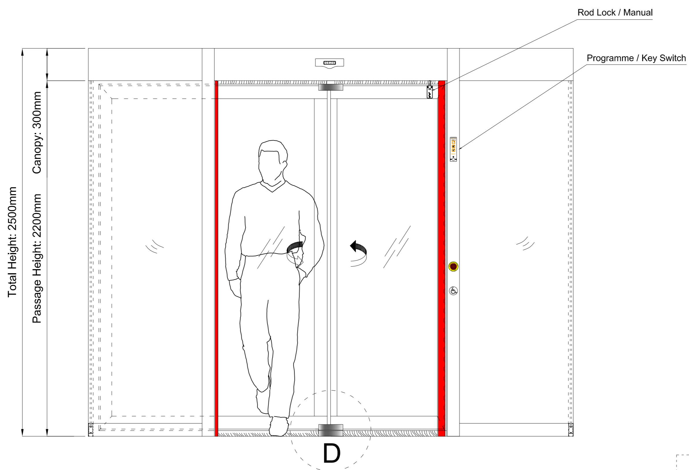
FRONT VIEW
